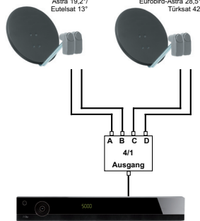
Beispiel 2: 4 Satelliten (Single-LNBs) Astra 19,2°/ Eutelsat 13° Eurobird-Astra 28,5°/ Türksat 42°
