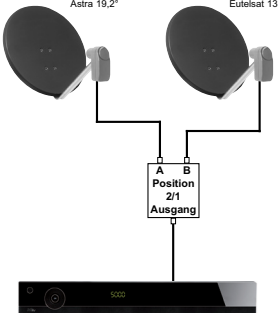
Beispiel 1: 2 Satelliten (Single-LNBs) Astra 19,2° Eutelsat 13°
